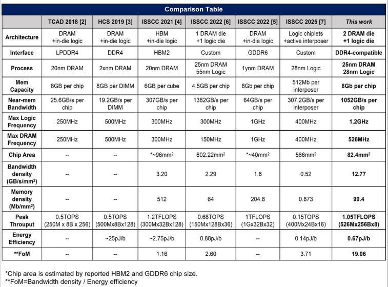
Figure 30.7.6: Comparison with prior works.
