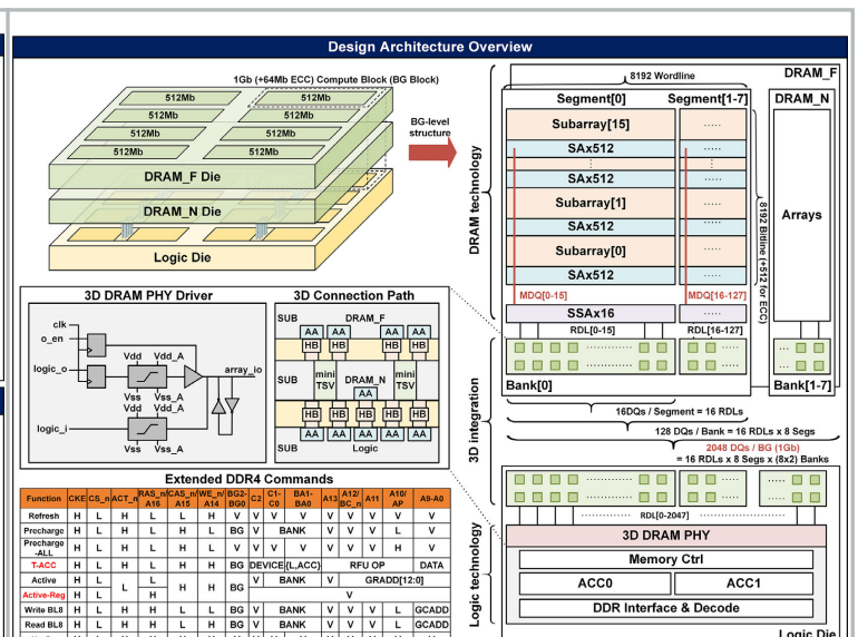
Figure 30.7.2: Overall design architecture and the extended DDR4 command list.
