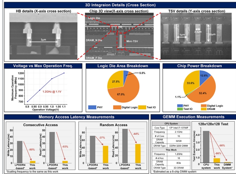
Figure 30.7.5: 3D integration details, area and power breakdown, and design measurements.
