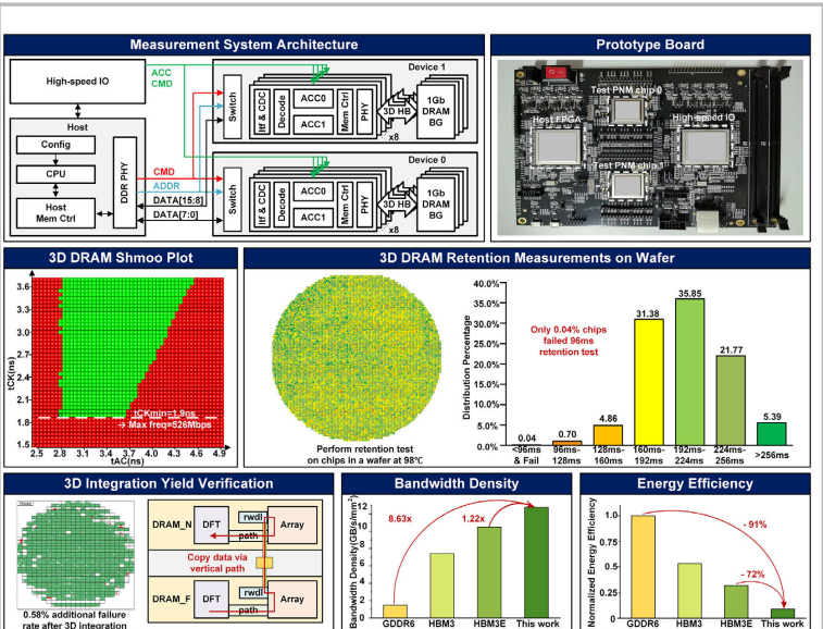
Figure 30.7.4: Measurement system architecture and 3D DRAM measurement results.
