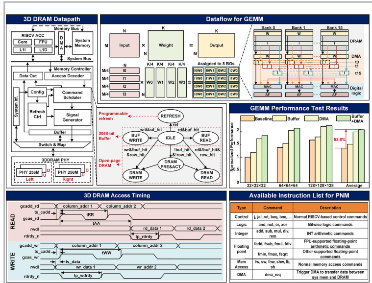
Figure 30.7.3: Datapath and access timing for 3D DRAM, and dataflow and performance test for GEMM.
