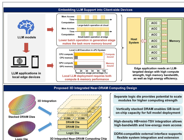
Figure 30.7.1: Client-side LLM application challenges and the presented 3D integrated near-DRAM computing design.
